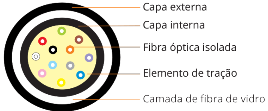
FIBER-LAN AR (PFV) 12F
